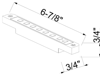
TS-A6000C OR TS-A6500C REPLACEMENT MODULE DIMENSIONS
