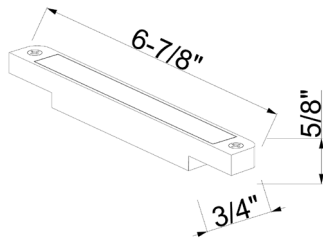
TS-A6000C OR TS-A6500C REPLACEMENT MODULE DIMENSIONS
